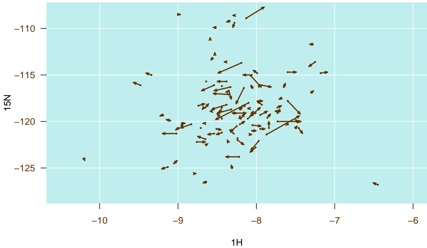
Peak movements, pH 4.5 vs. 7.0, HuPrP121-231
